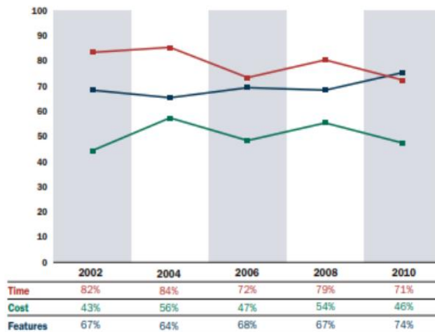
Fig. 6. Time and cost overruns, plus percentage of features delivered from CHAOS Research for the years 2002 to 2010
