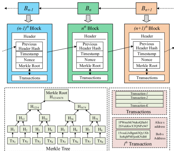
Fig. 2. Blockchain architecture.
